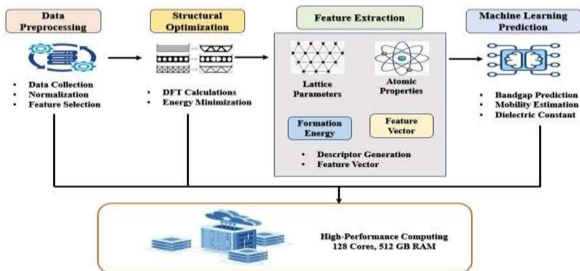
Figure 1. Computational workflow for materials design and property prediction Cs 2 AgTlBr 6
